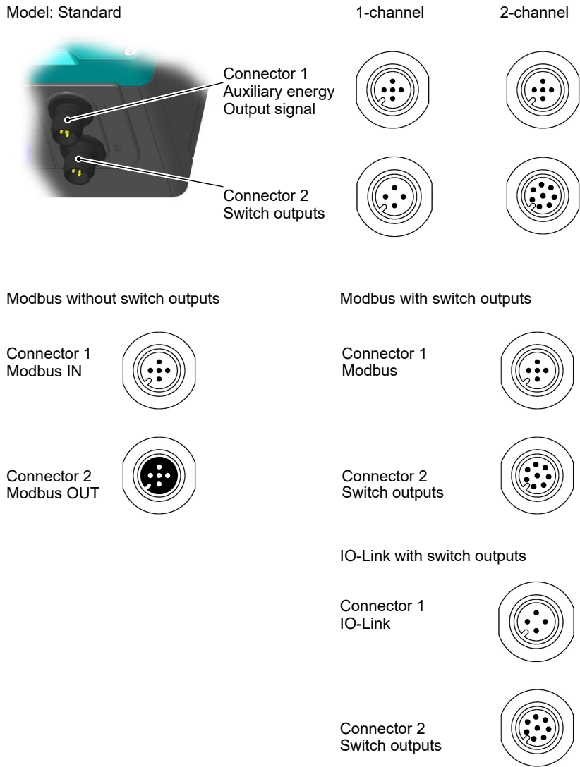
Fig. 3: Electric connections
