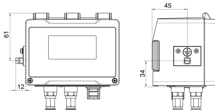
Fig. 7: Dimension drawing ATEX
