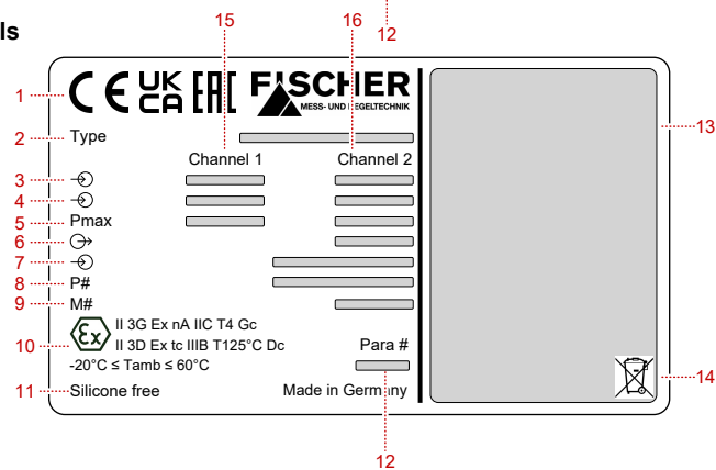
Fig. 5: Type plate
